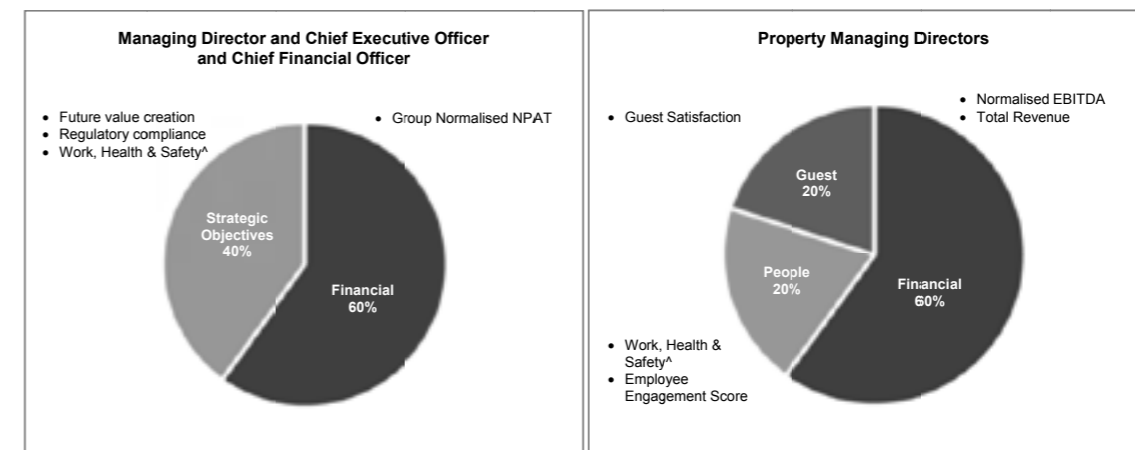
Figure 3: Weighted Scorecard
